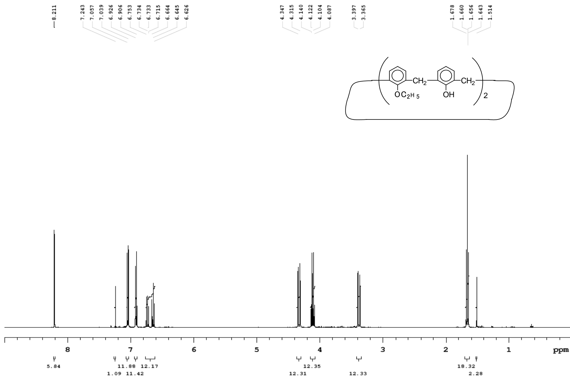
光譜二 ^1\text{H-NMR} (CDCl 3 ) spectrum of 25,27-Diethoxy-26,28-dihydroxycalix[4]arene (27)
