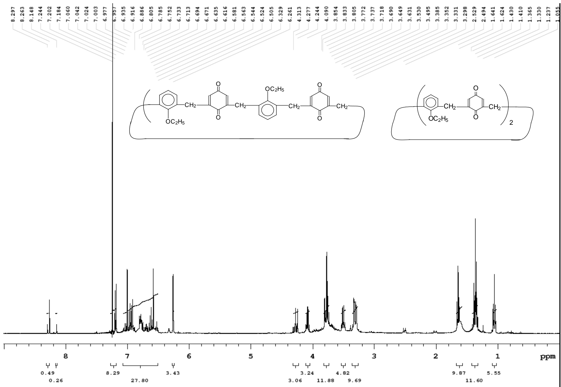
光譜三 ^1\text{H-NMR} ( \text{CDCl}_3 ) spectrum of 25,27-Diethoxy-26,28-calix[4]diquinone (32)、(33)
