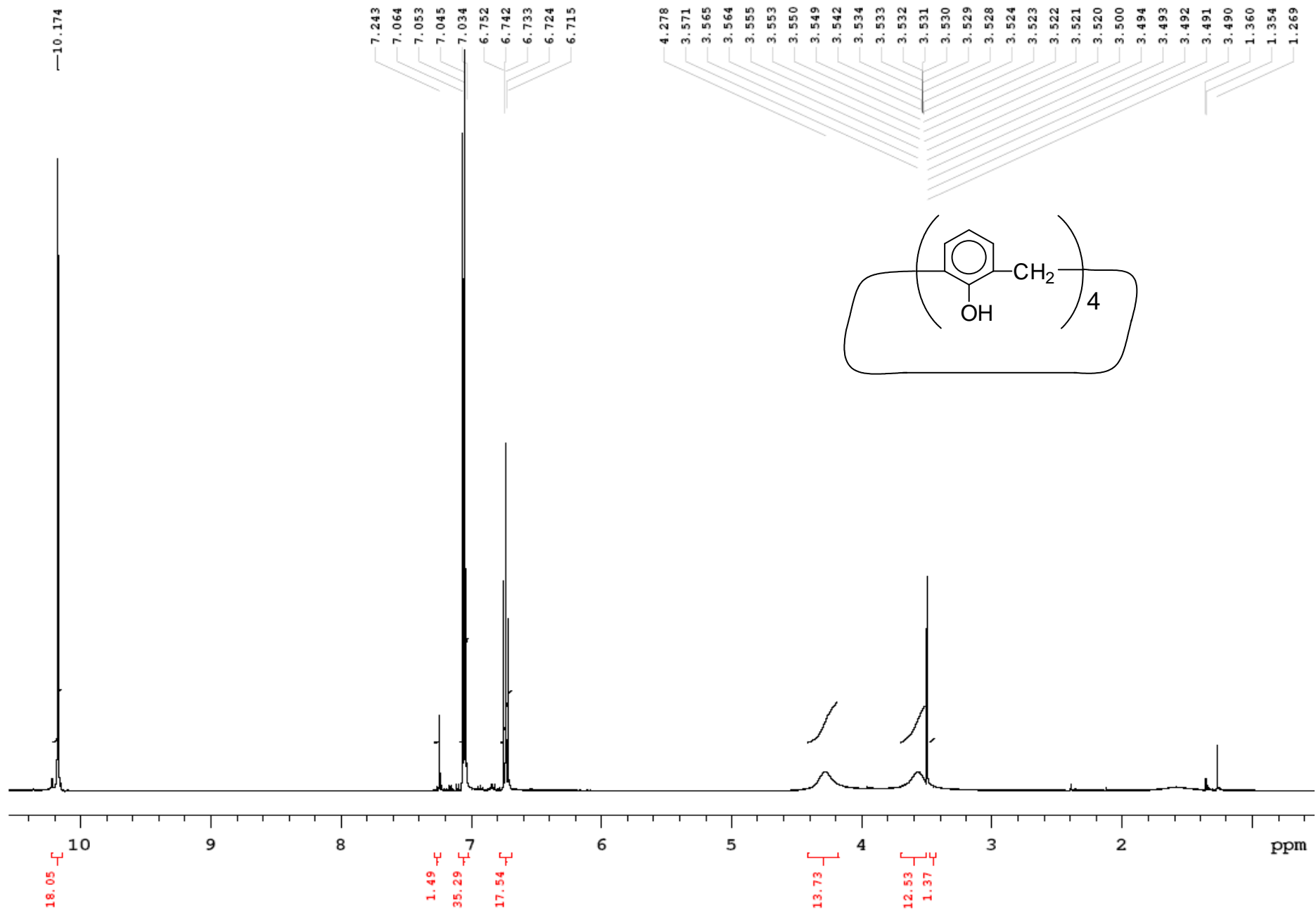
光譜— ^1\text{H-NMR} ( \text{CDCl}_3 ) spectrum of 25,26,27,28-Tetrahydroxycalix[4]arene (6)
